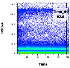
Time gate
